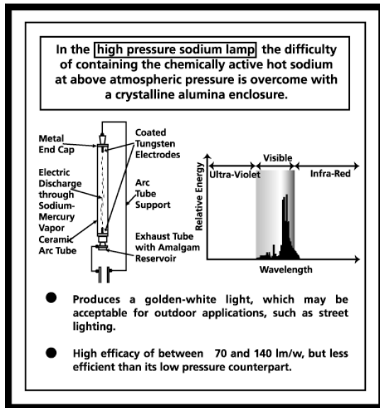
Figure 8.17: The high-pressure sodium lamp Figure 8.18: Comparison of mercury vapor, metal halide, and high-pressure sodium lamps
