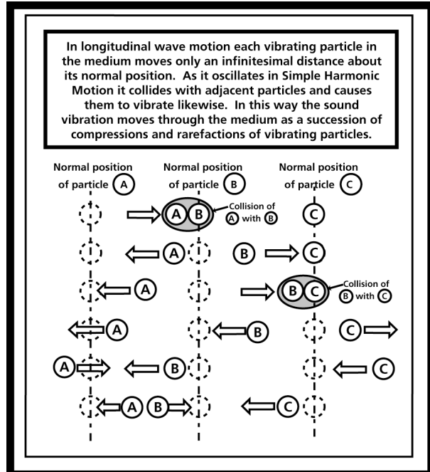
Figure 9.2: Propagation of sound
