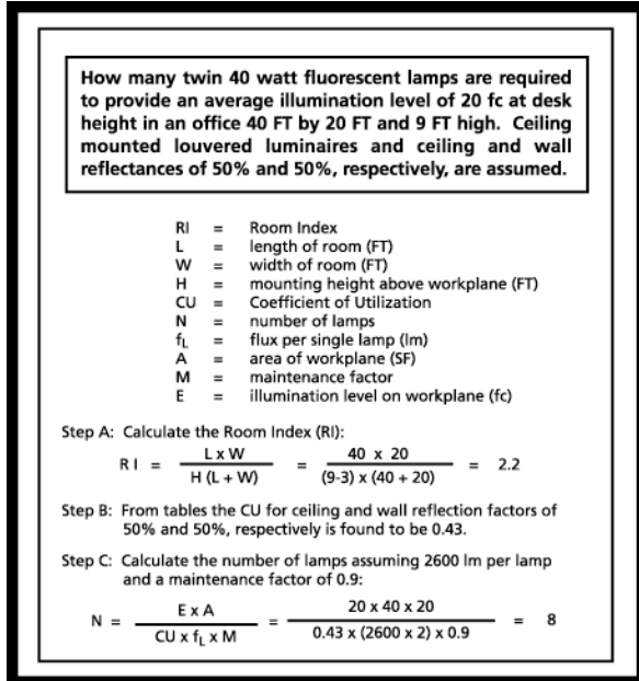
Figure 8.35: Number of lamps required for a given illumination level
