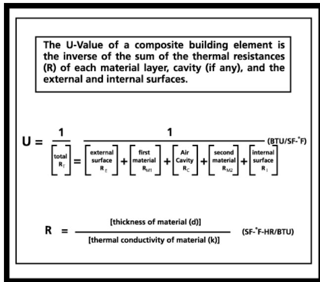
Figure 4.8: Calculation of the thermal transmittance or U-value of a construction assembly
