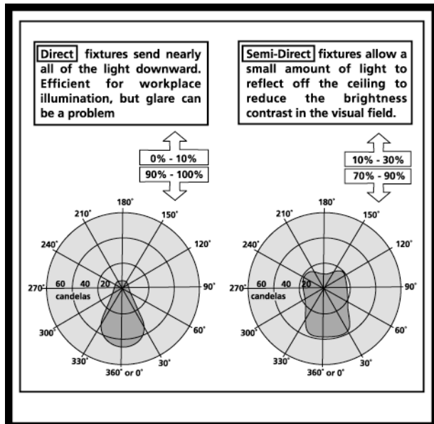
Figure 8.25: Direct and semi-direct luminaires
