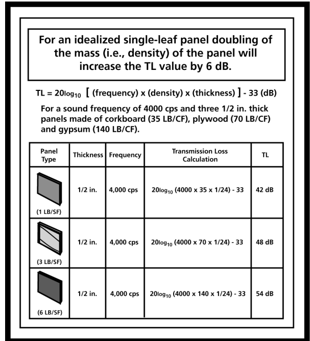
Figure 11.6: Effect of mass on a single-leaf panel
