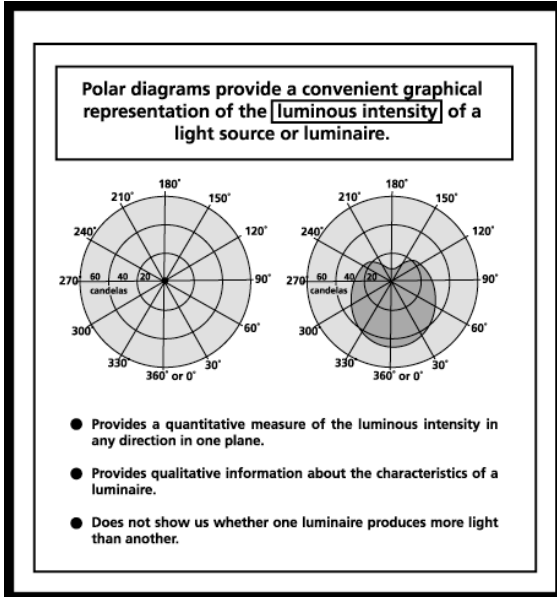
Figure 8.23: Polar diagrams
