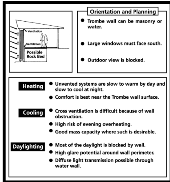
Figure 5.21: The Trombe Wall system
