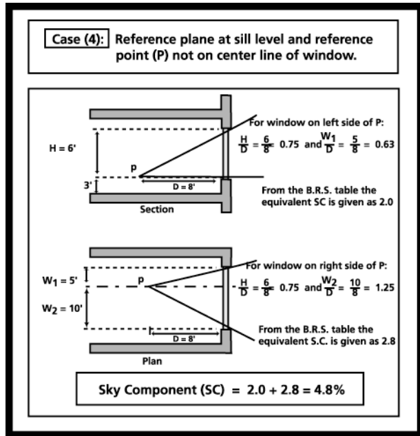
Figure 7.20: Case (4) – Reference Point not on center line of window
