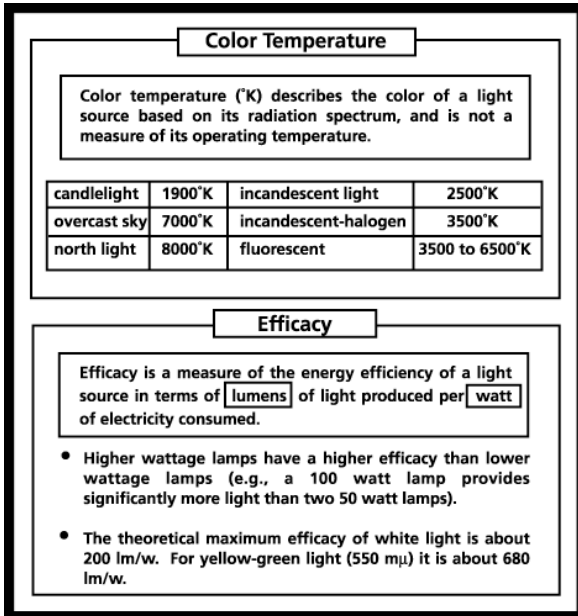
Figure 8.5: Color Temperature and Efficacy
