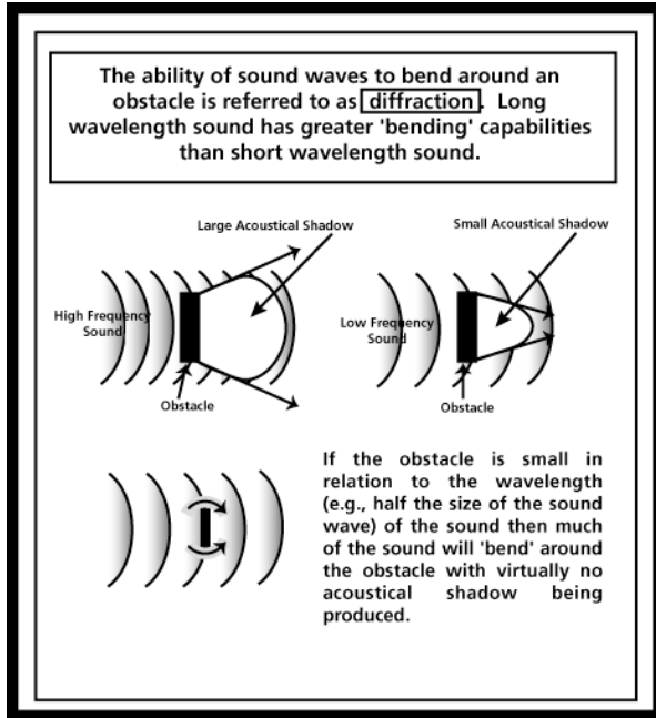
Figure 10.3: Acoustical shadows
