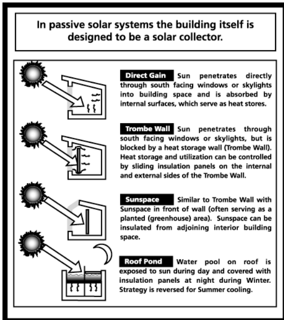
Figure 5.18: Typical passive solar systems
