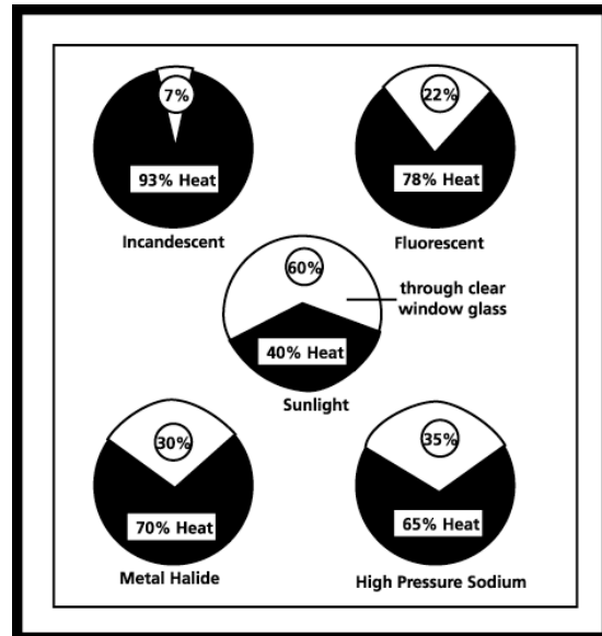
Figure 8.2: Efficiency of light sources
