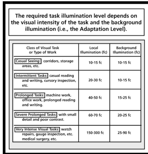
Figure 6.26: Typical illumination levels
