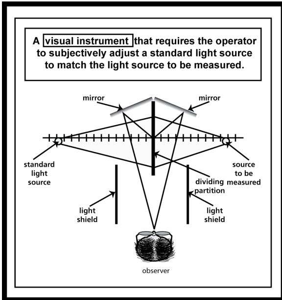
Figure 7.9: Photometer
