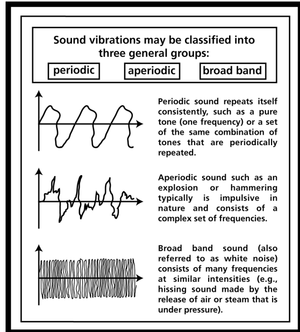
Figure 9.4: Types of sound vibration
