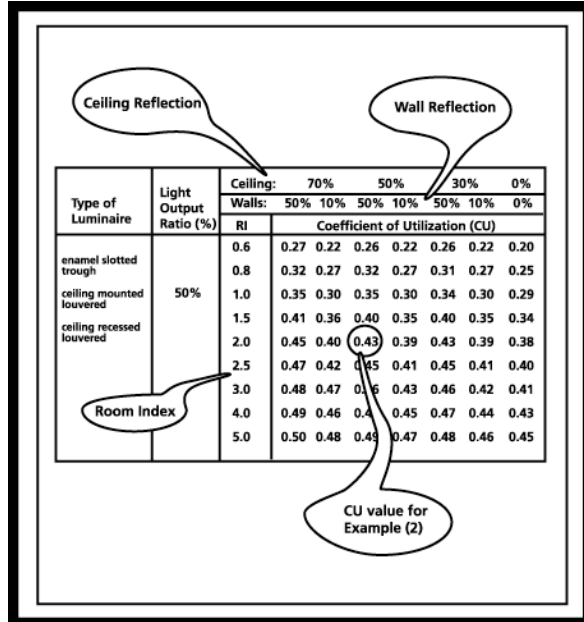
Figure 8.36: Looking up the CU value for the example shown in Figure 8.35
