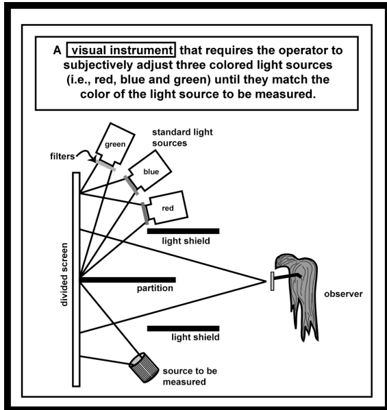
Figure 7.5: Colorimeter
