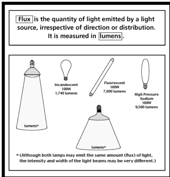
Figure 6.13: Light flux
