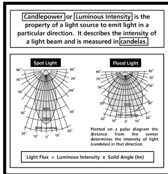
Figure 6.14: Luminous intensity
