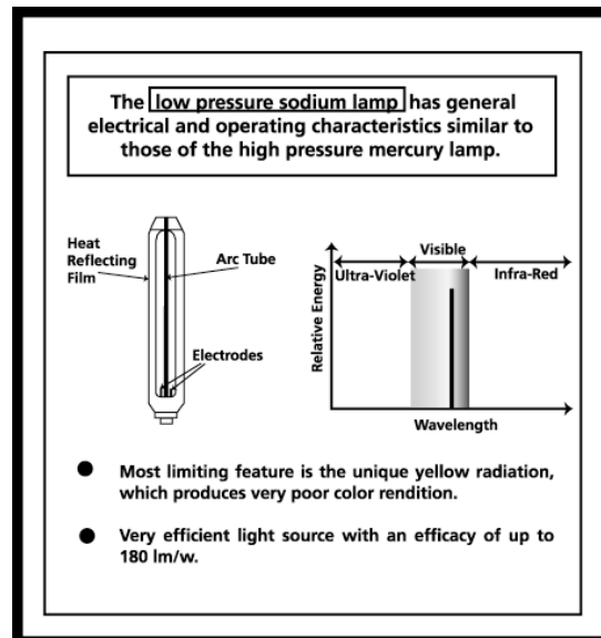
Figure 8.16: The low-pressure sodium lamp
