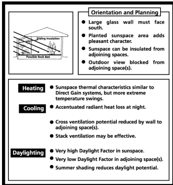
Figure 5.22: The Sunspace system
