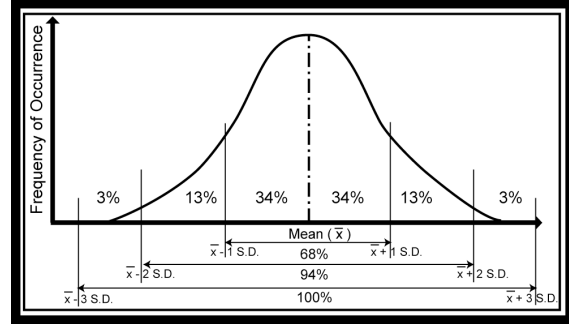
Figure 1.6: Standard Deviations
