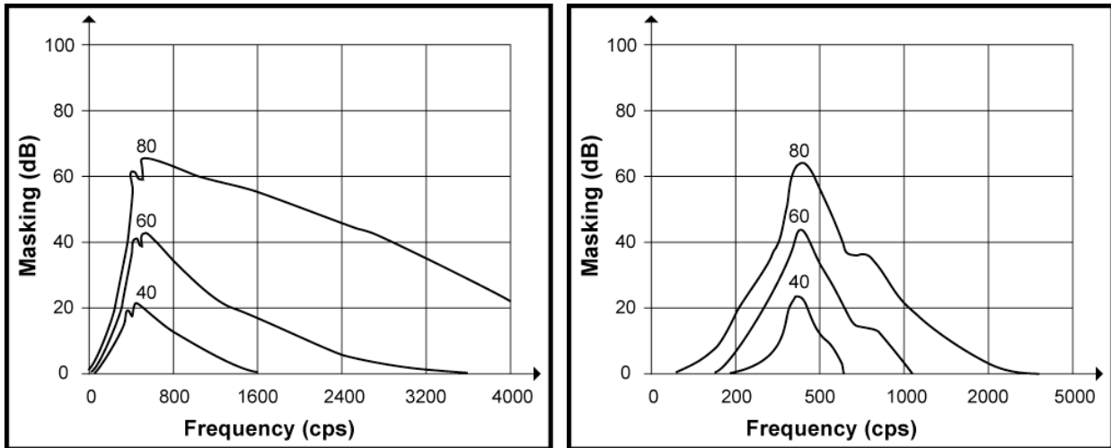
Figure 10.14: Masking effect of a pure tone Figure 10.15: Masking effect of a narrow band
