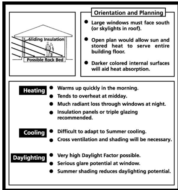
Figure 5.19: The Direct Gain system
