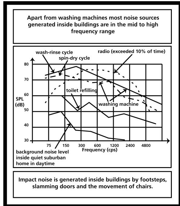
Figure 11.28: Residential noise sources
