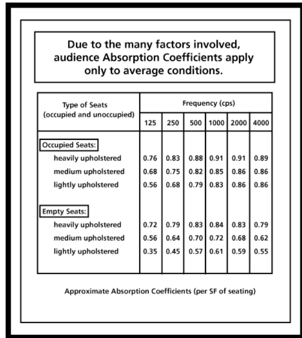
Figure 10.20: Absorption due to audience (according to Beranek 1996)
