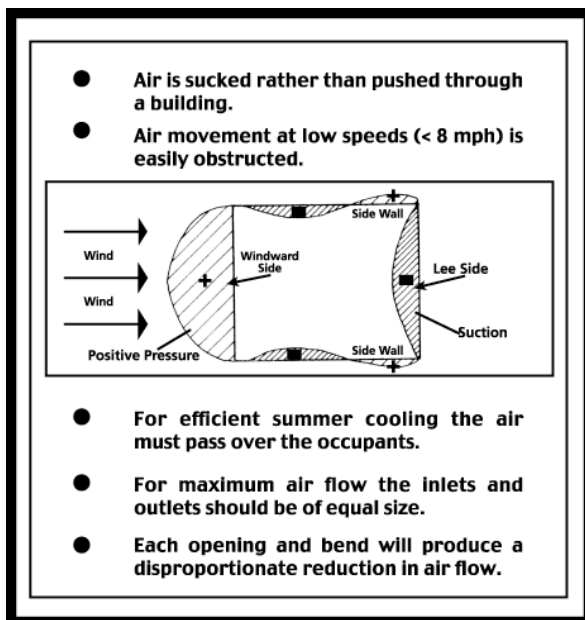
Figure 3.21: Impact of wind on buildings
