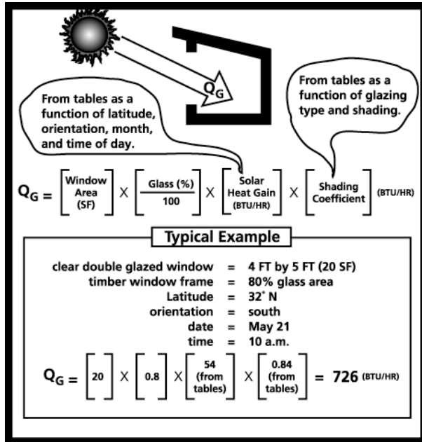
Figure 5.20: Solar heat gain through glass
