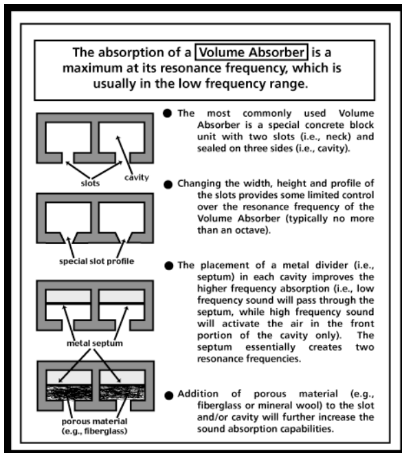
Figure 10.11: Different configurations of a concrete block absorption unit
